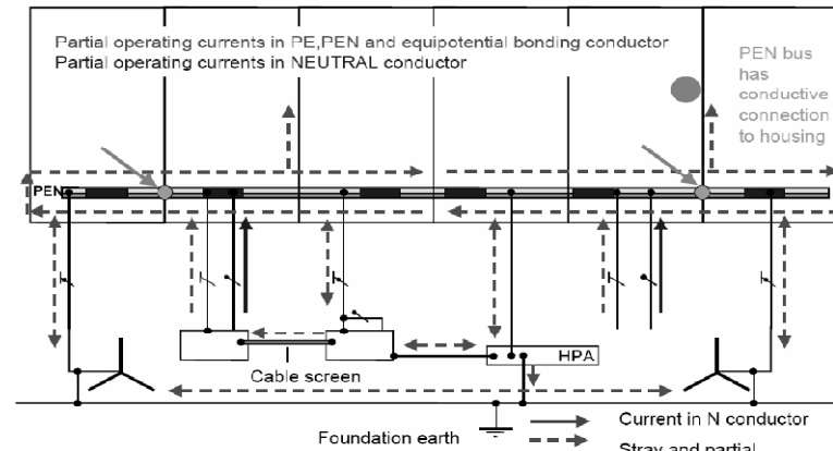
Low voltage main distribution
